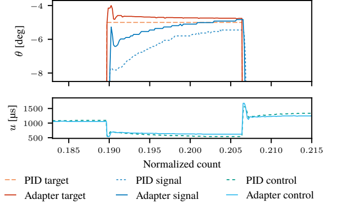
Fig. 24: A close-up from the 0.5–0.5mm perforation with target adapter. The signal response generally resembles that of Figure 10 from the simulated problem.
