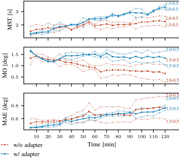
Fig. 21: Metrics evolution over the 2h duration of the experiment for KOSs in a higher state of degradation (1.5–0.5mm and 2–0.5mm perforations, see annotations), with their average overlayed. Each point represents the calculated value of the metric on identical 5min sequences of targets. Plots for all metrics and numerical values can be found in Figure C.4 and Table C.IV, respectively.
