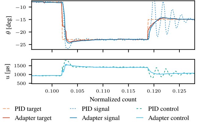
Fig. 25: A close-up from the slow-aggressive PID controller with target adapter. The manner in which the target is adapted resembles that of Figure 8 from the simulated problem.
