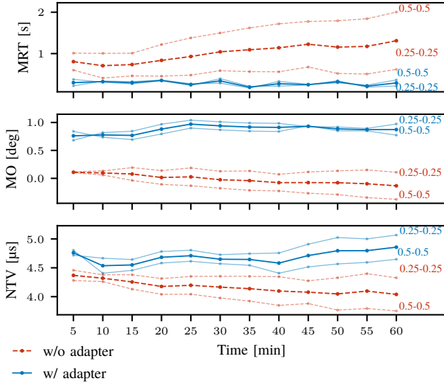
Fig. 19: Metrics evolution over the 1h duration of the experiment for KOSs in a lower state of degradation (0.25–0.25mm and 0.5–0.5mm perforations, see annotations), with their average overlayed. Each point represents the calculated value of the metric on identical 5min sequences of targets. Plots for all metrics and numerical values can be found in Figure C.3 and Table C.III, respectively.
